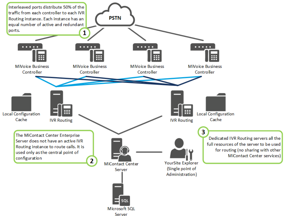
Figure 122: High availability configuration
